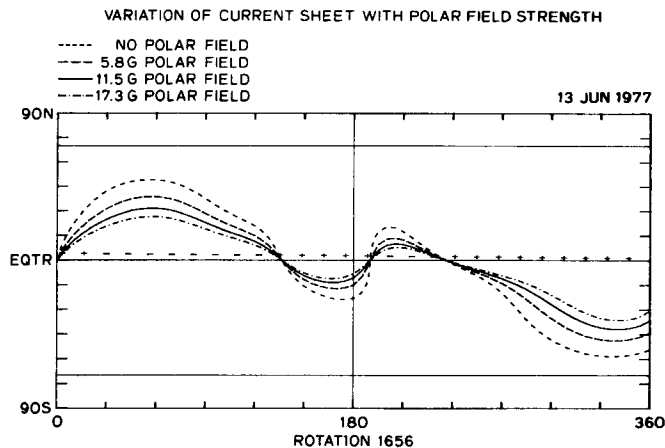
Fig. 6. Computed heliospheric current sheets on Carrington rotation 1656, beginning June 13, 1977, for several values of added solar polar magnetic field. As the strength of the polar field is increased, the computed current sheet approaches the plane of the solar equator.
