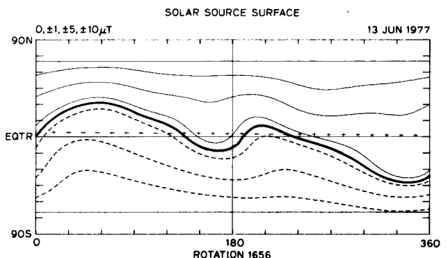
Fig. 2. The same format as Figure 1 but for a later Carrington rotation, 1656, beginning June 13, 1977. Note that the latitudinal extent of the computed heliospheric current sheet extends to higher latitudes than in Figure 1.
