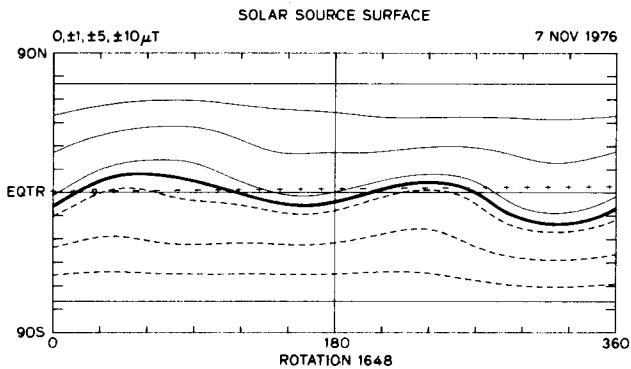
Fig. 1. Computed magnetic field contours on a spherical source surface concentric with the sun at a radius of 2.35 R_S for Carrington rotation 1648, beginning November 7, 1976. The solid contour lines represent field directed away from the sun with observed field strengths 1, 5, and 10 \mu\text{T} ; the dashed contours represent field directed toward the sun. The observed field strengths should be multiplied by a factor of 1.8 to account for magnetograph saturation [Svalgaard et al. , 1978]. The heavier line near the solar equator is where the direction of the computed field changes from away to toward and is assumed to be the source of the heliospheric current sheet. The + and - symbols represent daily values of the polarity of the interplanetary magnetic field observed at the earth, adjusted for the 5-day transit time of solar wind from the sun to the earth.
