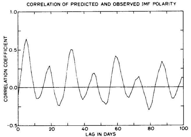
Fig. 9. Cross correlation between the IMF polarity predicted from the adopted computation of the heliospheric current sheet and the polarity observed at the earth. The lag of the first peak is 5 days, which represents the transit time from the sun to the earth of the solar wind near the sector boundaries.
